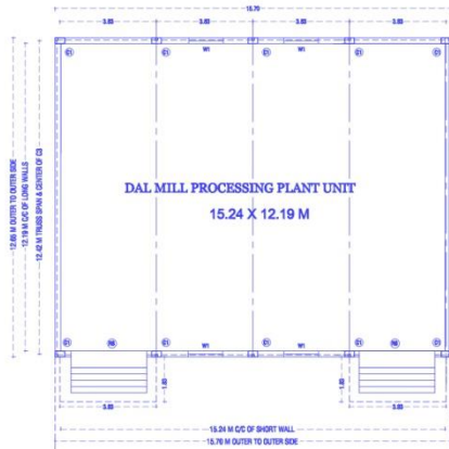
DAL MILL PROCESSING PLANT UNIT PLAN
